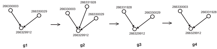
Fig. 4. An example of the sequential patterns extracted using AMW-gSpan algorithm
