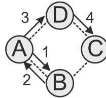
Fig. 2 Sample run of RW (numbered directed edges indicate progress of the random walk)
