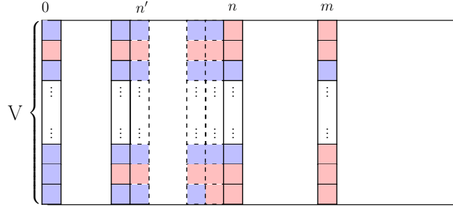
Fig. 5: Illustration of Algorithm 1. The blue vertices at time i denote the winning region W_i for Player 1. The times n, n' \in N and Pre_1 computation at change point n increases the winning region but is stable at time n' .
