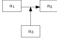
Fig. 3. Extended Argumentation: A attacks B, C attacks the attack
