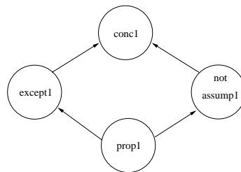
Figure 1: AF after proponent's arguments are put forward
