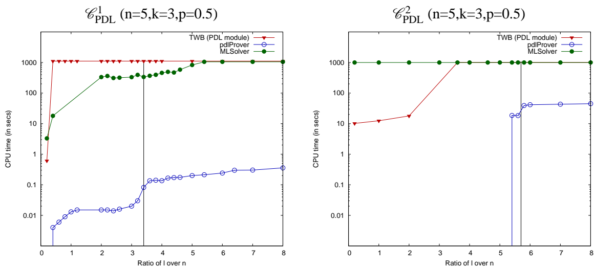
Figure 2: Performance of the decision procedures
