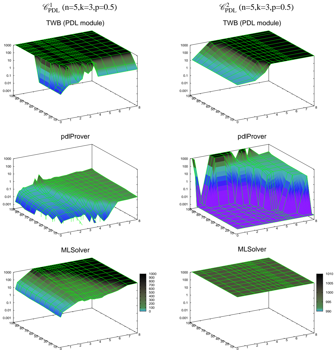
Figure 3: CPU time percentile graphs
