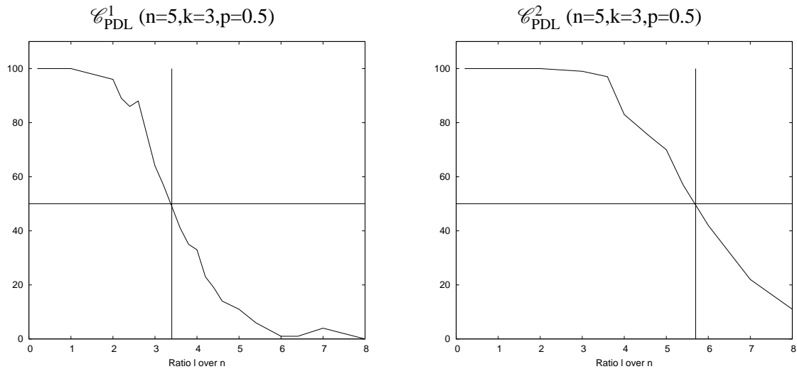
Figure 1: Satisfiability of formulae in \mathcal{C}_{PDL}^1 and \mathcal{C}_{PDL}^2
